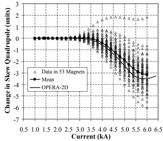
Fig. 3-9. Current dependence of the skew quadrupole component.
