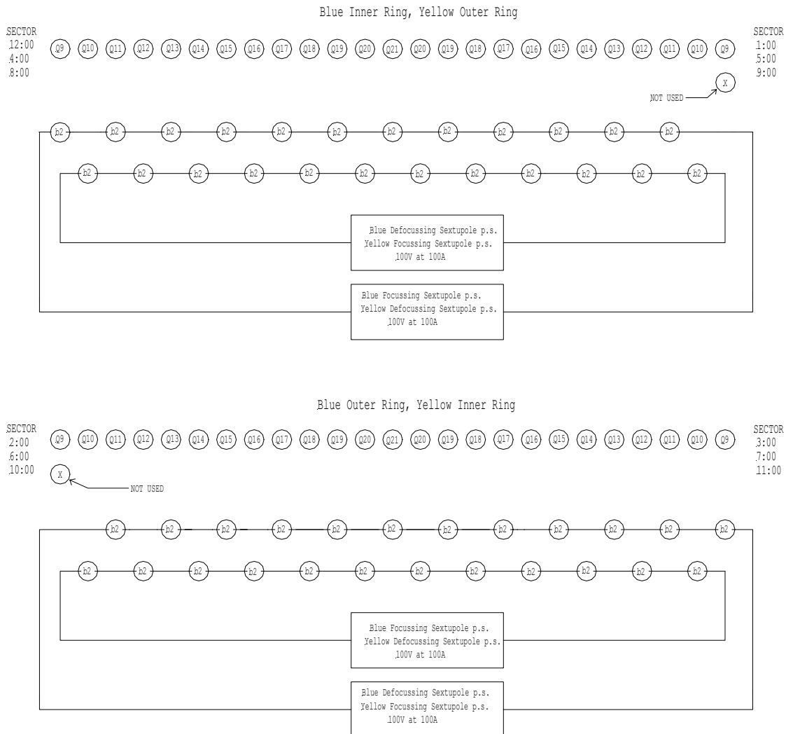
Fig. 2-12. Sextupole circuit.
