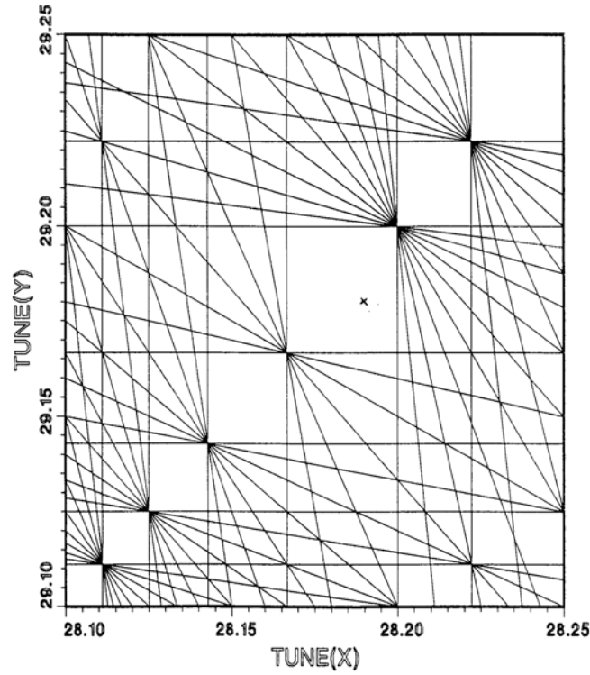
Fig. 11-15. Tune diagram showing the selected working point of RHIC at v_x = 28.19 , v_y = 29.18 with neighboring sum and difference resonances.
