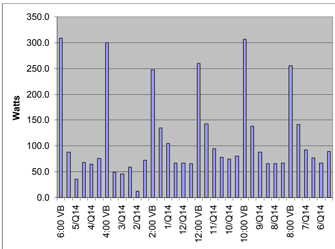
Figure 3-1 .Actual Heat Load Distribution in Blue Ring
