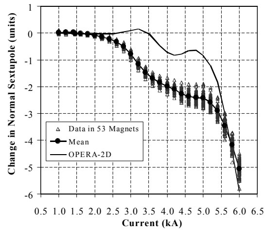
Fig. 3-10. Current dependence of the normal sextupole component.
